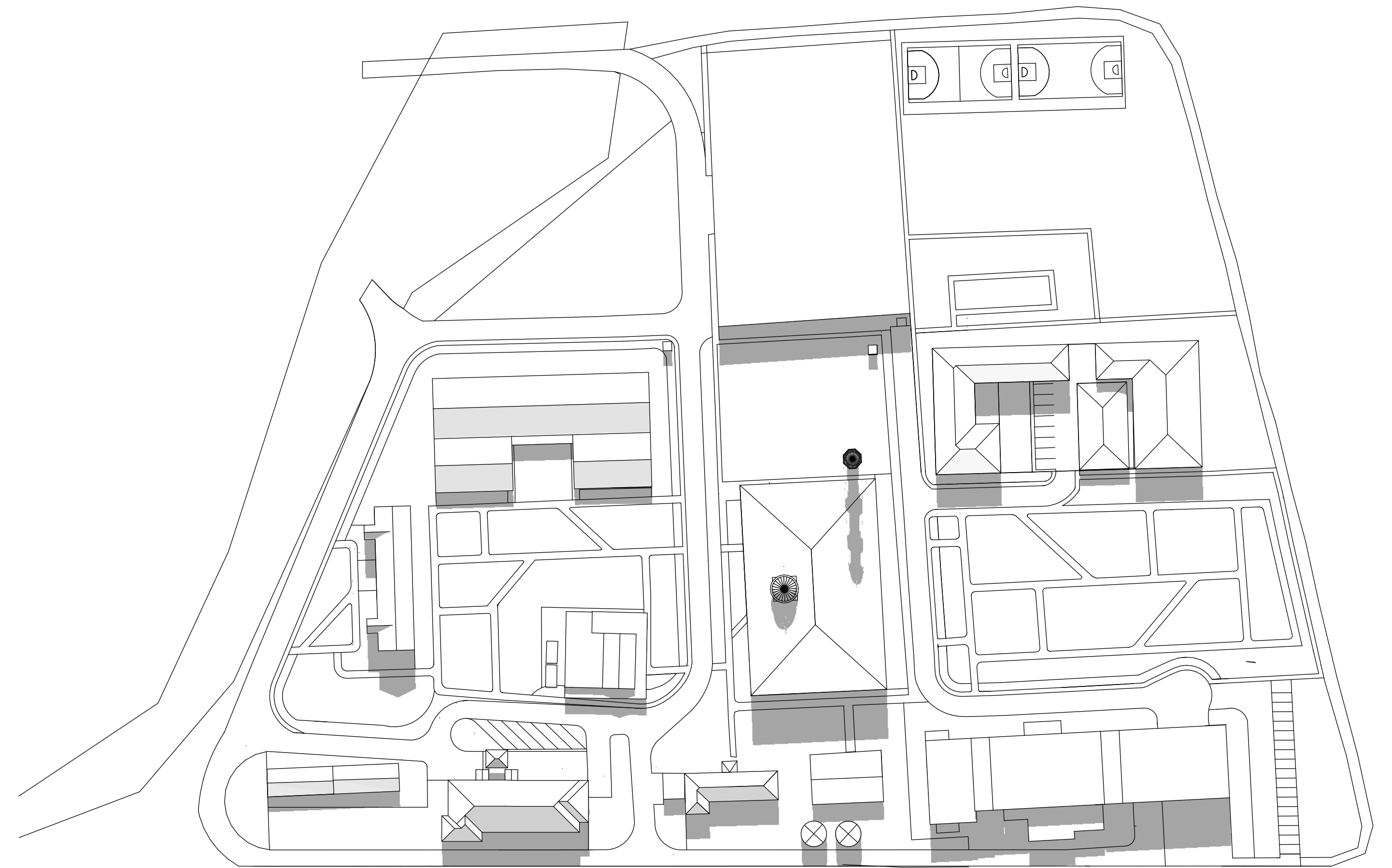
SHADOW DIAGRAM AT 12:00 PM 21ST JUNE
