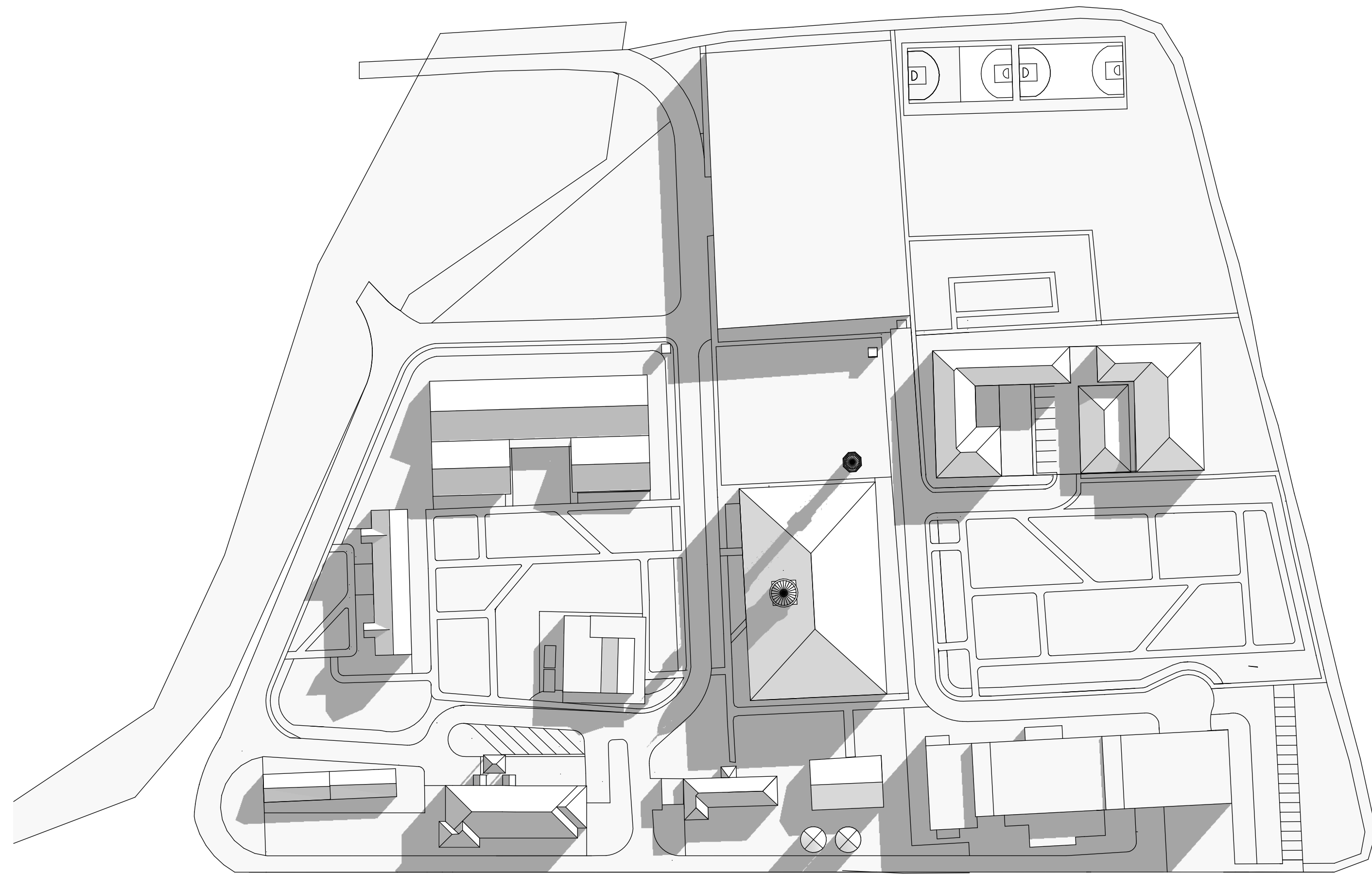
SHADOW DIAGRAM AT 9:00 AM 21ST JUNE
