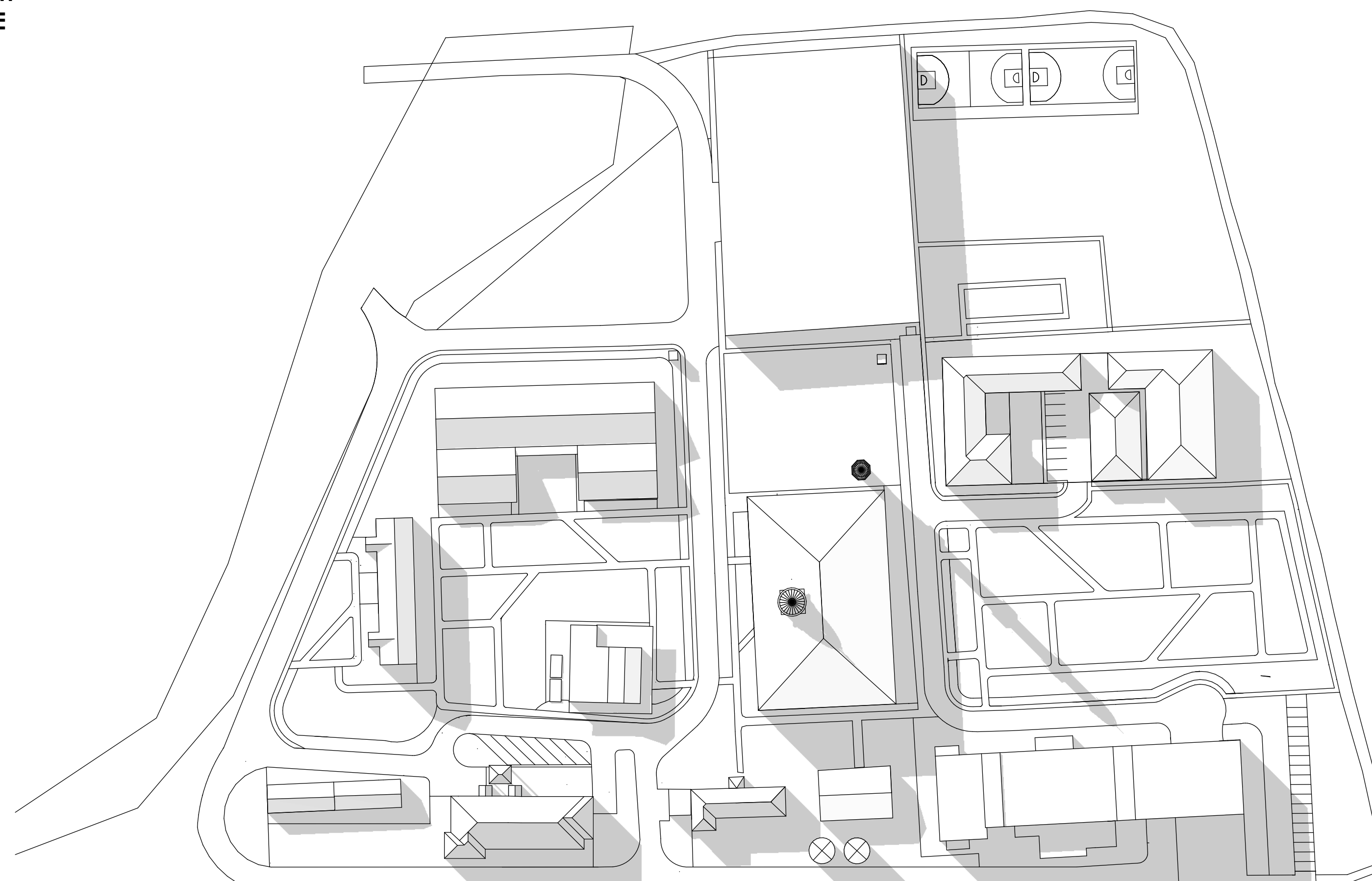
SHADOW DIAGRAM AT 3:00 PM 21ST JUNE
